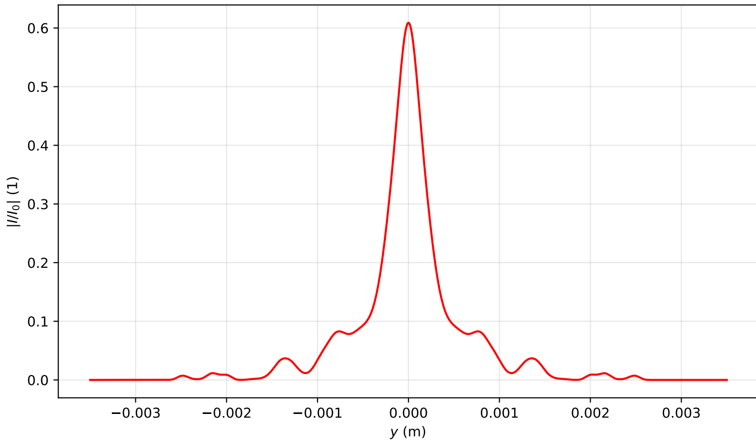
Intensity profile I(x=0, y, z=2.388)/I_0 , P_{in}=5.0P_{cr} , artificial time
